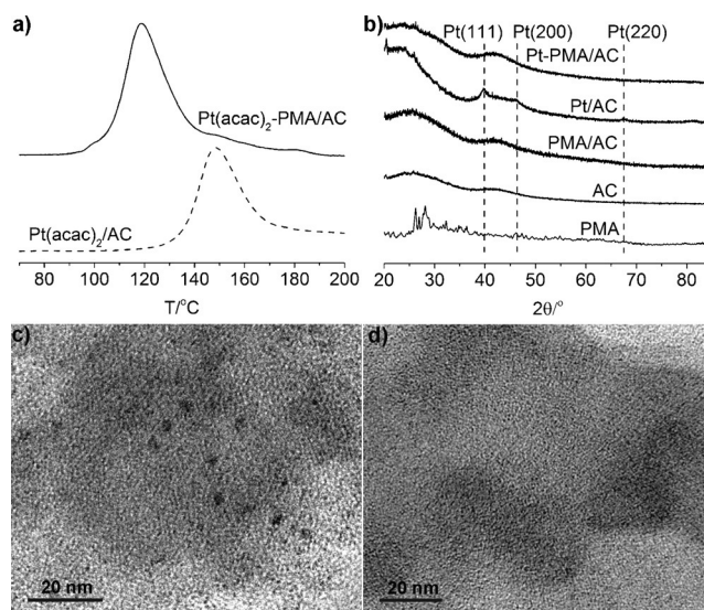
Figure 2. a) TPR profiles of \text{Pt}(\text{acac})_2\text{/AC} and \text{Pt}(\text{acac})_2\text{-PMA/AC} . Reduction conditions: 5 % \text{H}_2 in \text{N}_2 , 100 mL \text{min}^{-1} , 10 °C \text{min}^{-1} heating rate (70–200 °C), catalyst (50 mg). Before heating, the sample was stabilized in 5 % \text{H}_2 in \text{N}_2 at 70 °C for 60 min. b) XRD patterns of PMA, AC, \text{PMA/AC} , \text{Pt/AC} , and \text{Pt-PMA/AC} . The predicted diffraction peaks for Pt metal are indicated with dashed lines. A typical TEM image of c) \text{Pt/AC} and d) \text{Pt-PMA/AC} .
